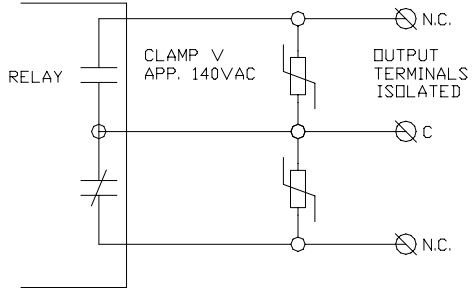
Typical ICM-HDIO-22P Output Circuit
