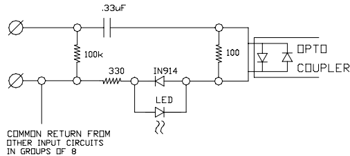
Typical ICM-HDIO-22P Input Circuit
