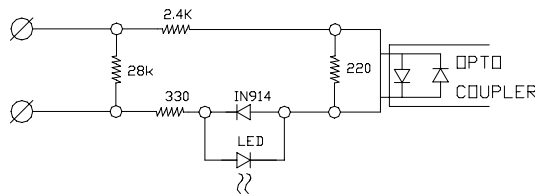
Typical ICM-HDIO-14P Input Circuit
