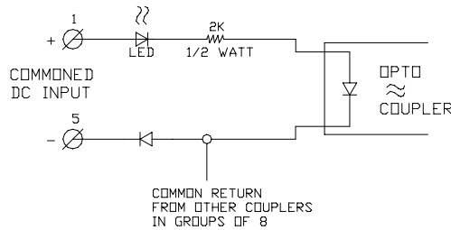
Typical ICM-HDIO-08P Input Circuit
