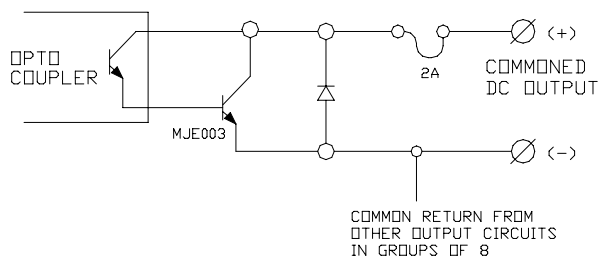
Typical ICM-HDIO-08P Output Circuit
