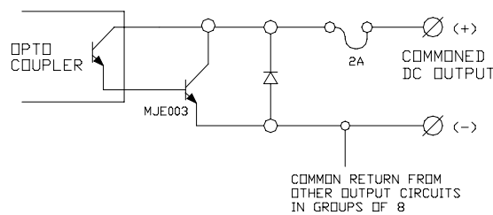
Typical ICM-HDIO-06P Output Circuit
