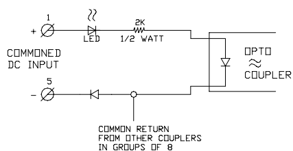
Typical ICM-HDIO-06P Input Circuit
