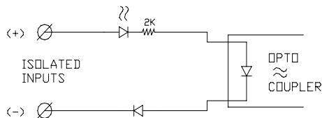
Typical ICM-HDIO-02P Input Circuit
